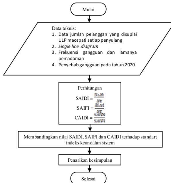
Gambar 1. Flowchart Penelitian
